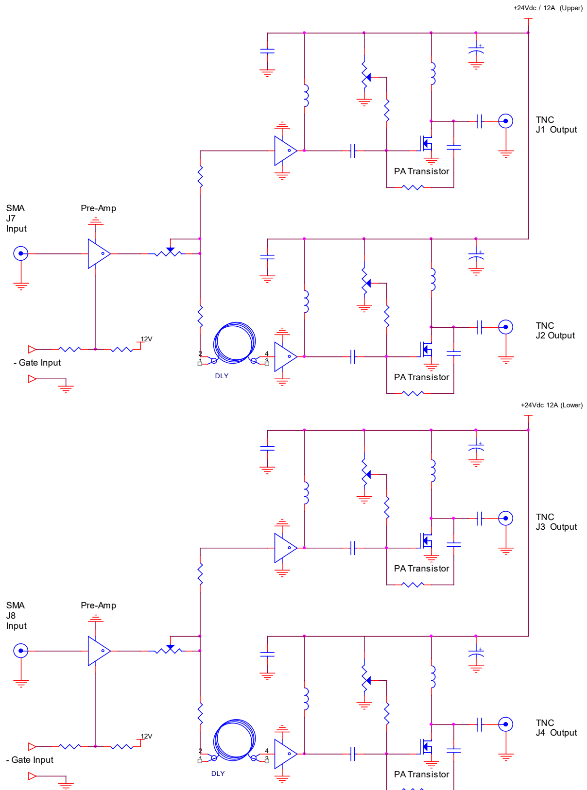
Figure 2: Driver Block Diagram
